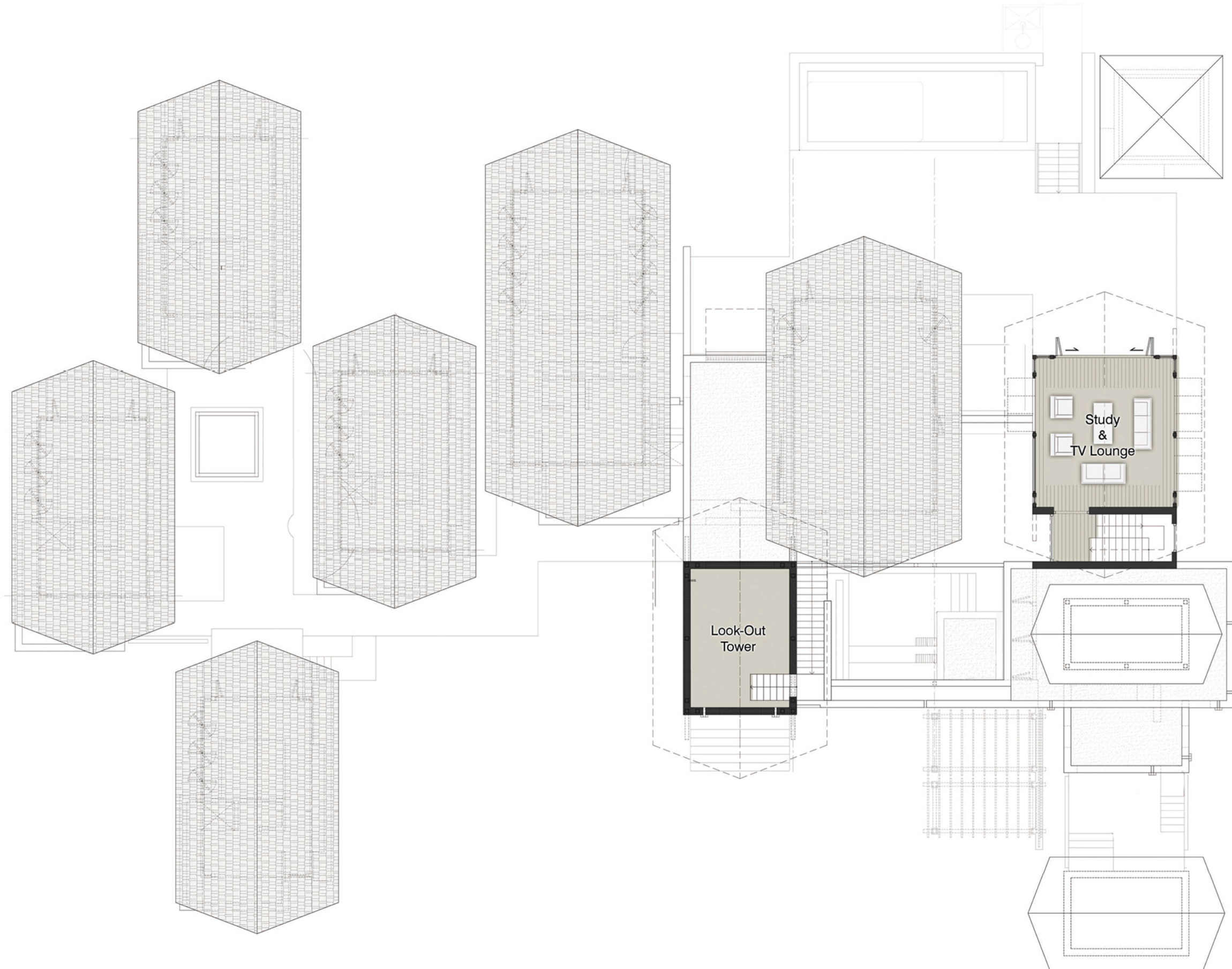
VILLA KIPILA FIRST FLOOR PLAN
