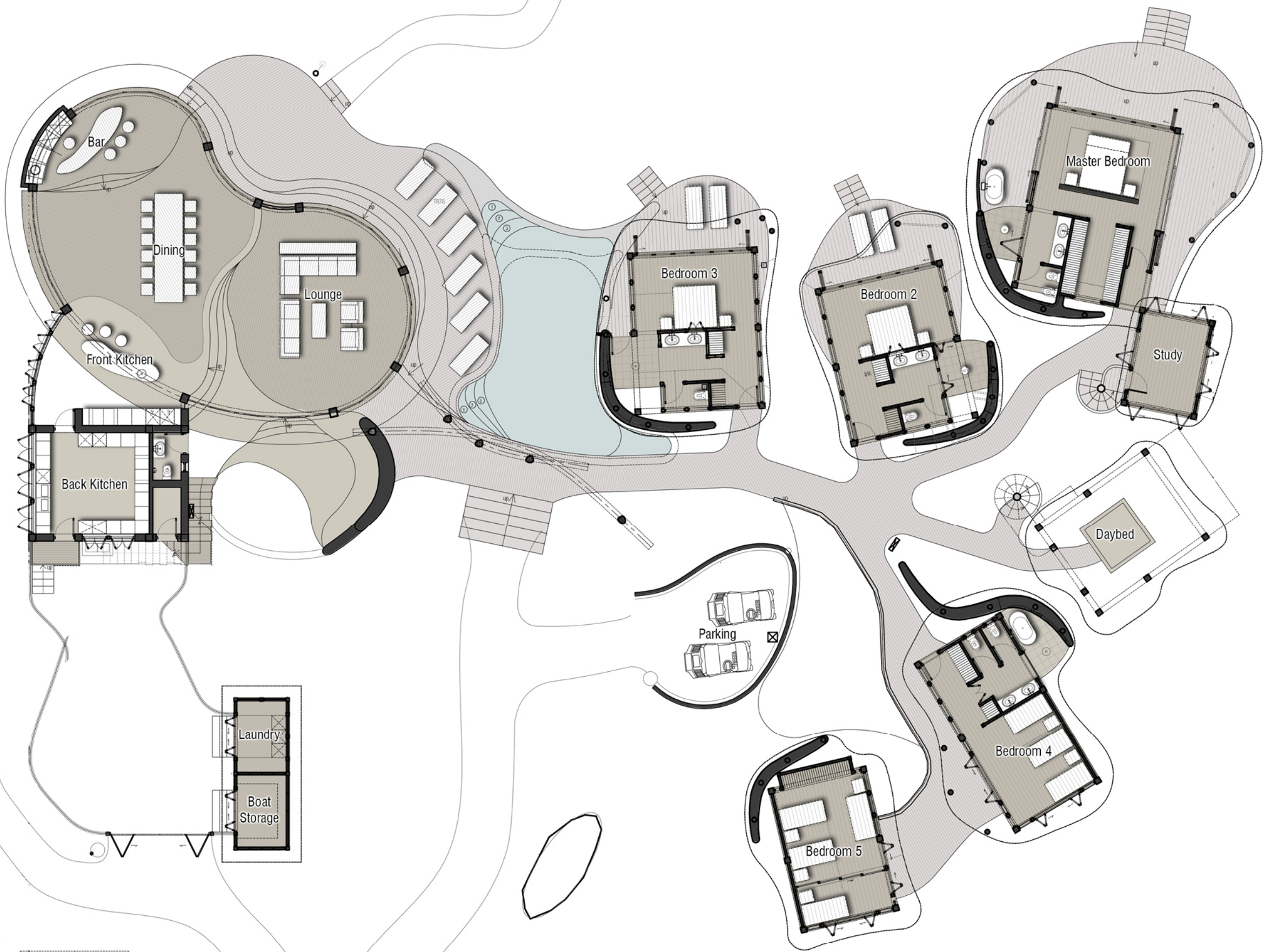
VILLA CASAMINA GROUND FLOOR PLAN
